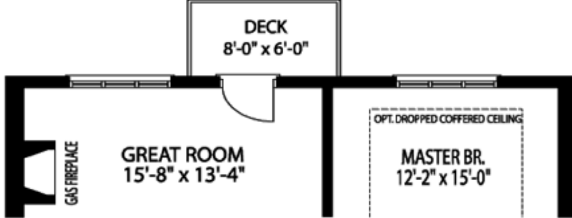
GROUND FLOOR ( W.O.B. - A & B CONDITION)
