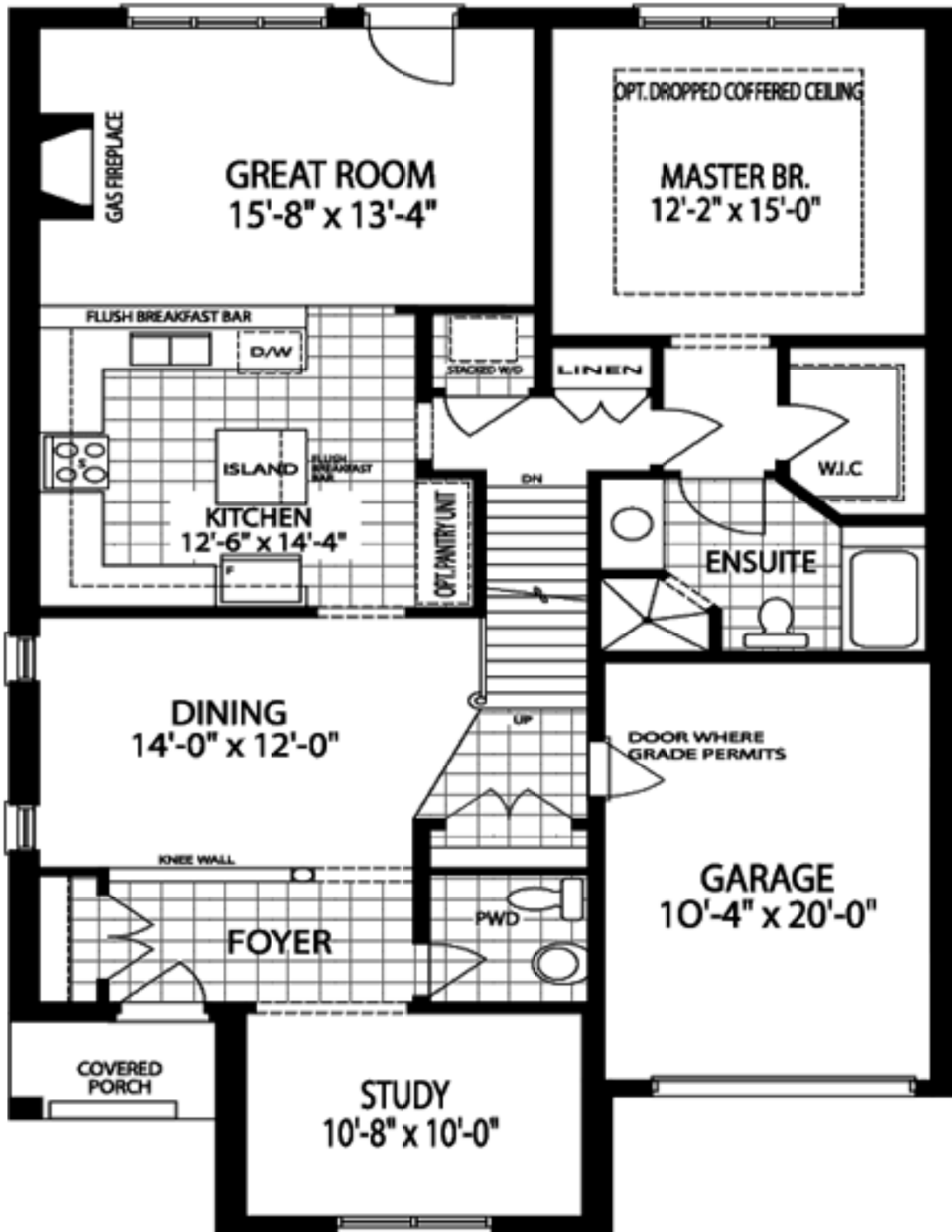
The Leithfield Ground Floor Plan B
