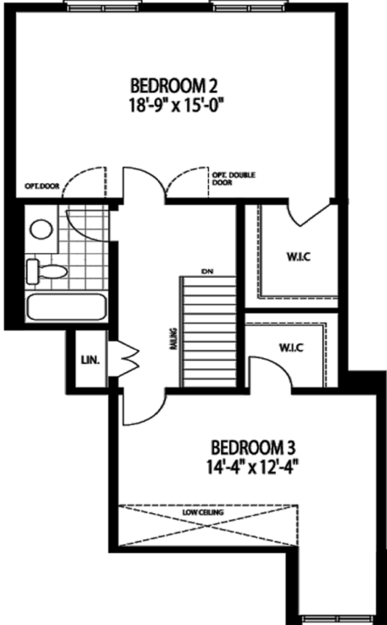
The Leithfield Upper Floor Plan A
