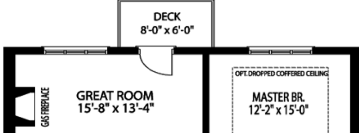
GROUND FLOOR ( W.O.B. - A & B CONDITION)
