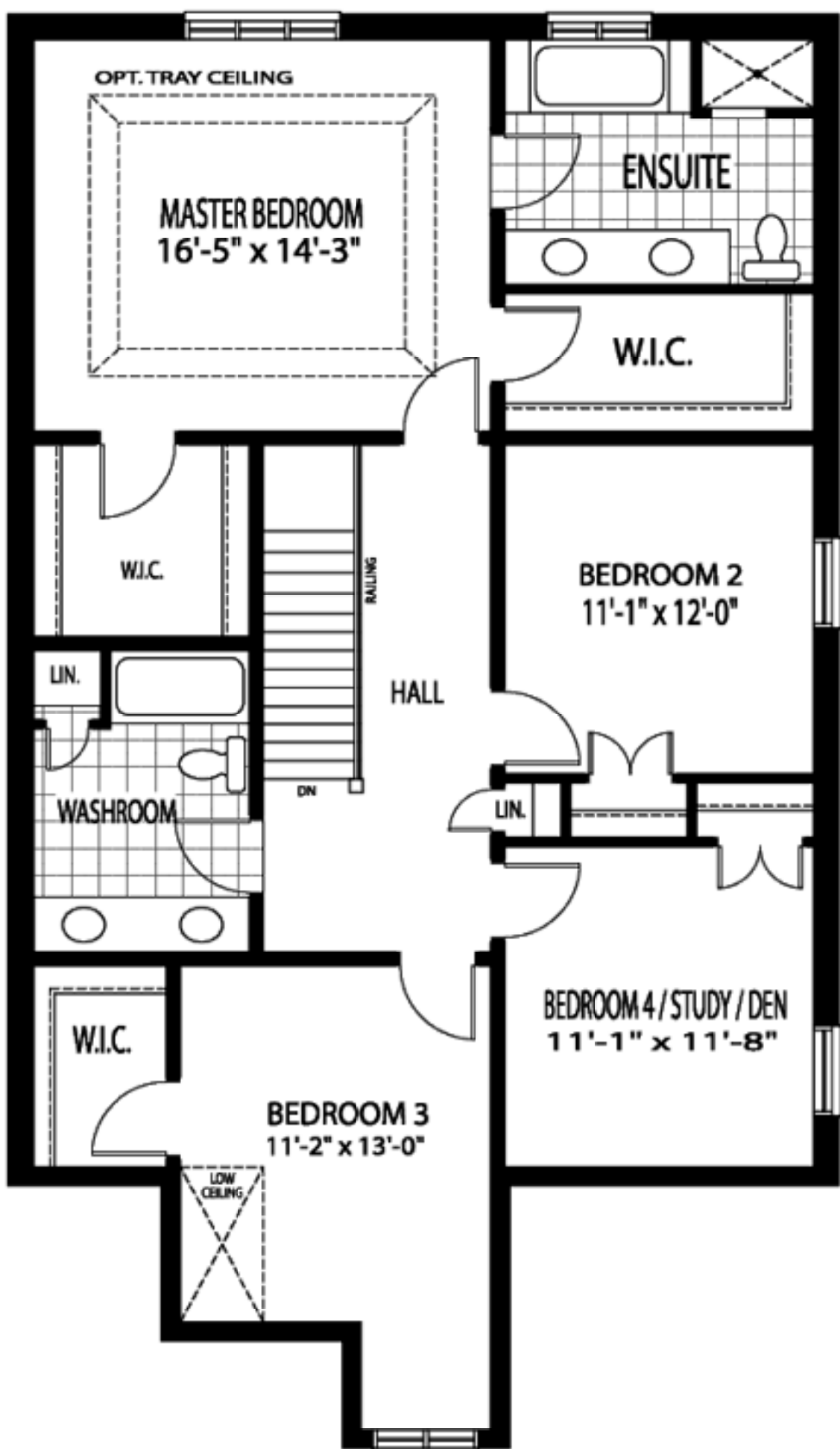
The Inverness 2nd Floor Plan A
