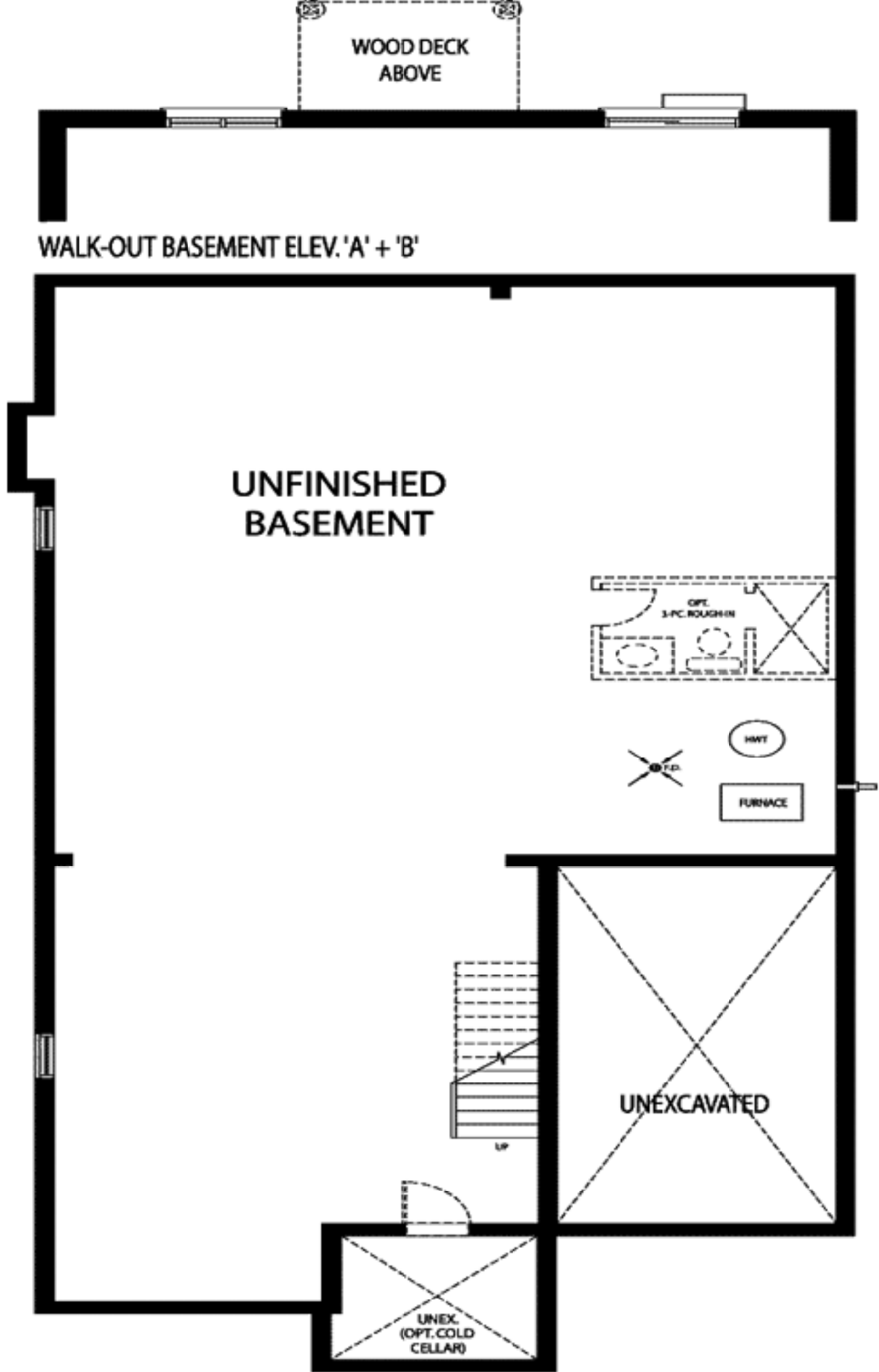
BASEMENT FLOOR PLAN 'A' & 'B'
