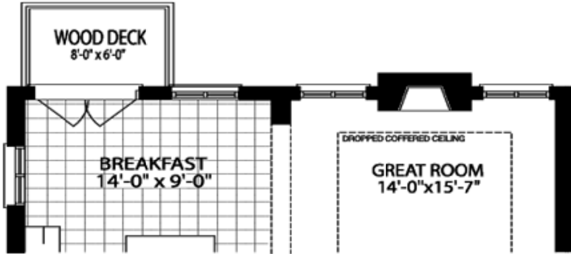
GROUND PLAN EL. 'A' + 'B' (WALK OUT CONDITION)
