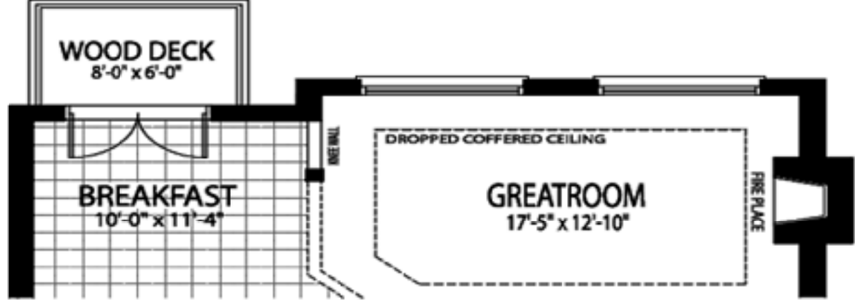
GROUND FLOOR ( W.O.B. - A & B CONDITION)
