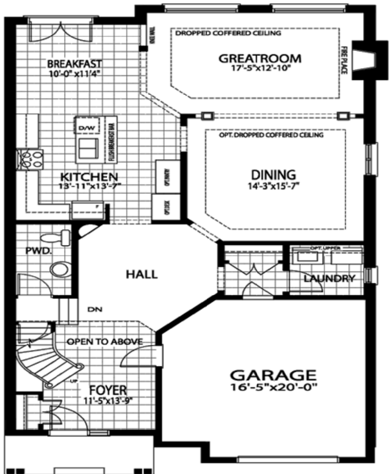
The Edinburgh Basement Floor Plan A
